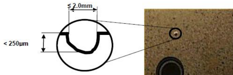
Figure 6: Etching hole (shallower than the substrate) in a MiniSKiiP's bottom surface
