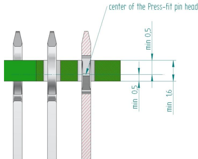
19. Figure: Press-in depth in PCB
