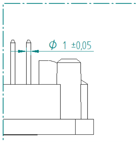
4. Figure: Solder pin diameter
