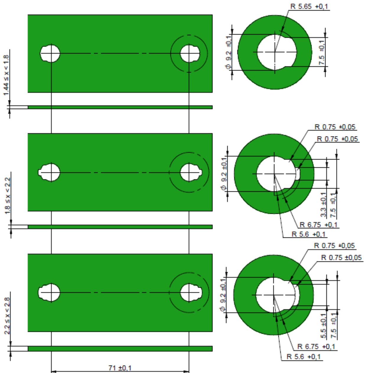
5. Figure: PCB-cutouts for two-clip modules at various board thickness
