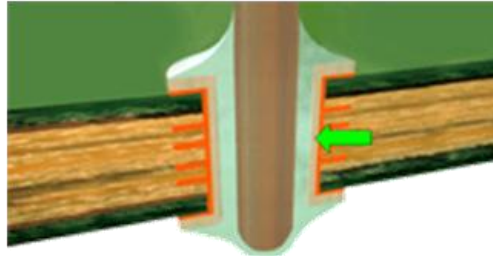
32. Figure: Plated through hole, good soldering
