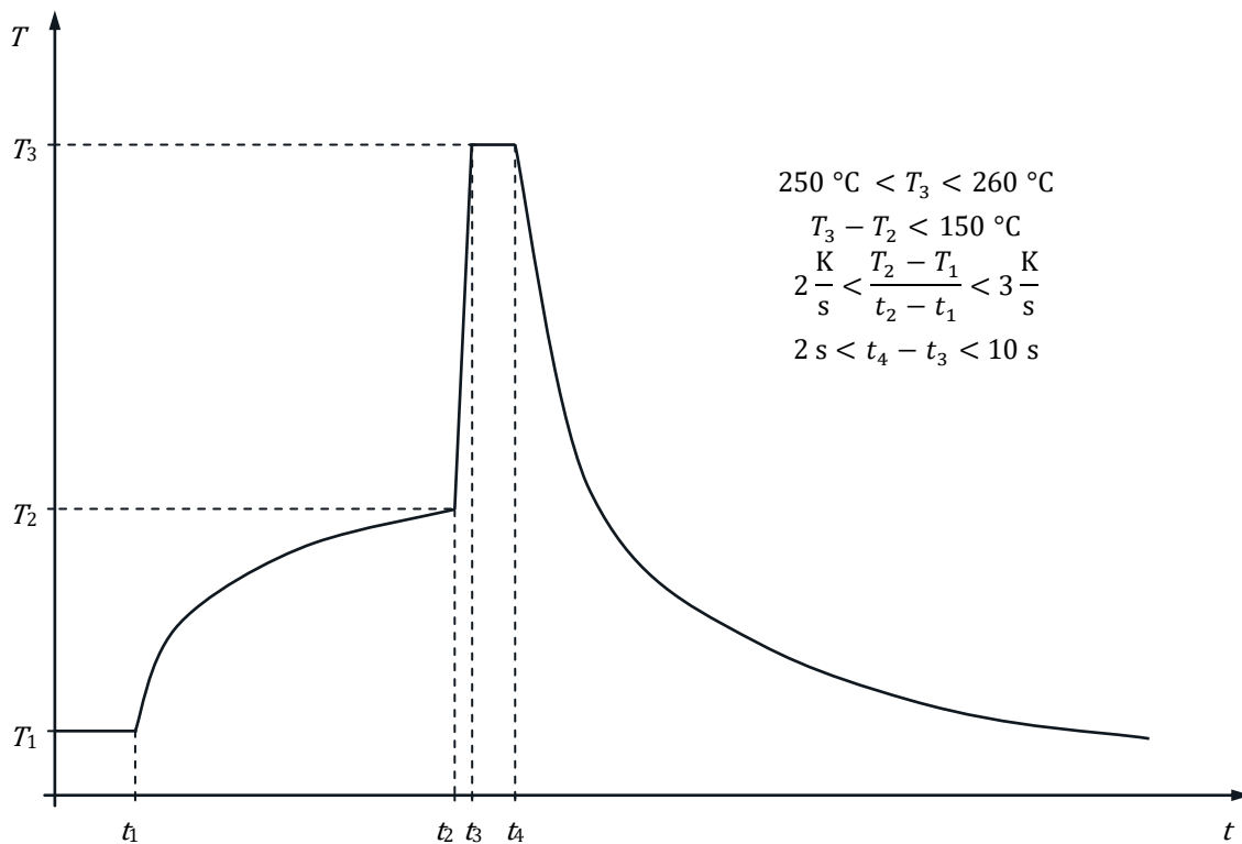
33. Figure: Typical profile for wave soldering
