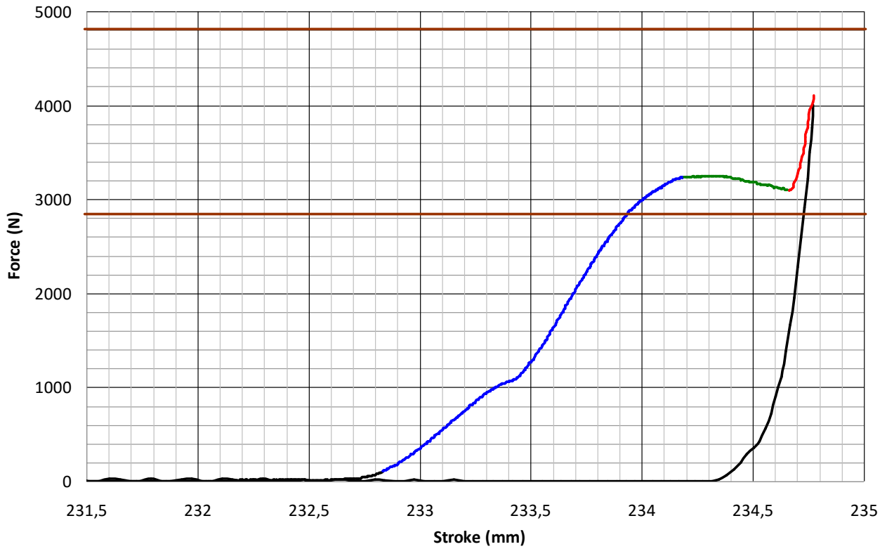
20. Figure: Typical press-in diagram of a 33 pin module
