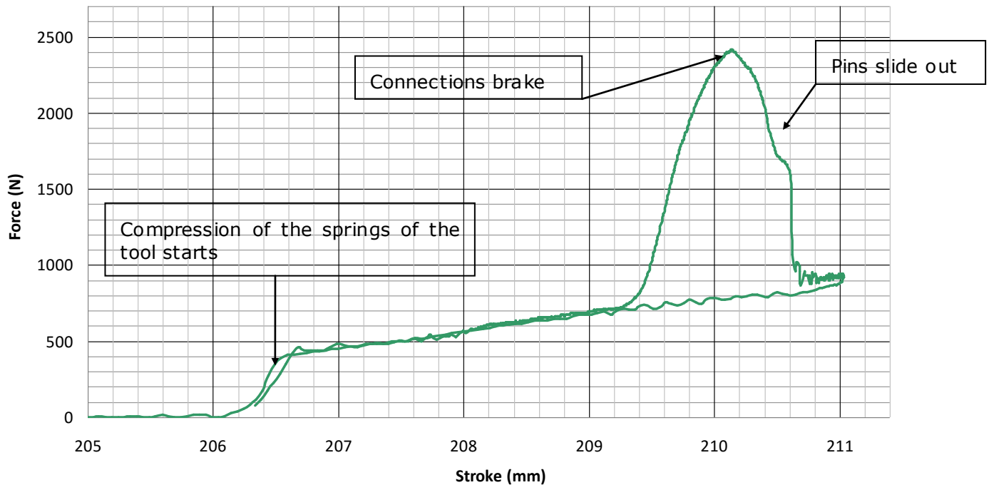
25. Figure: Force-path diagram of the press-out process
