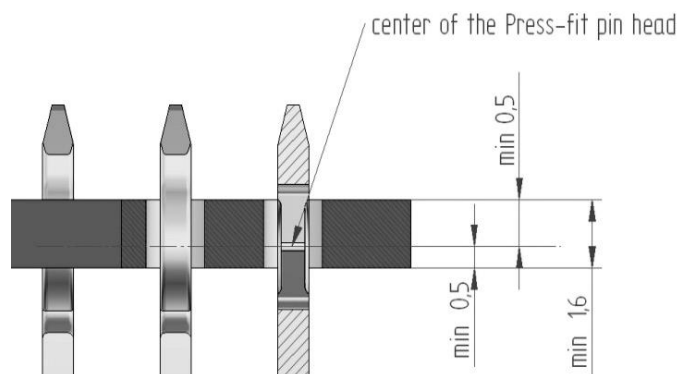
19. Figure Press-in depth in PCB
