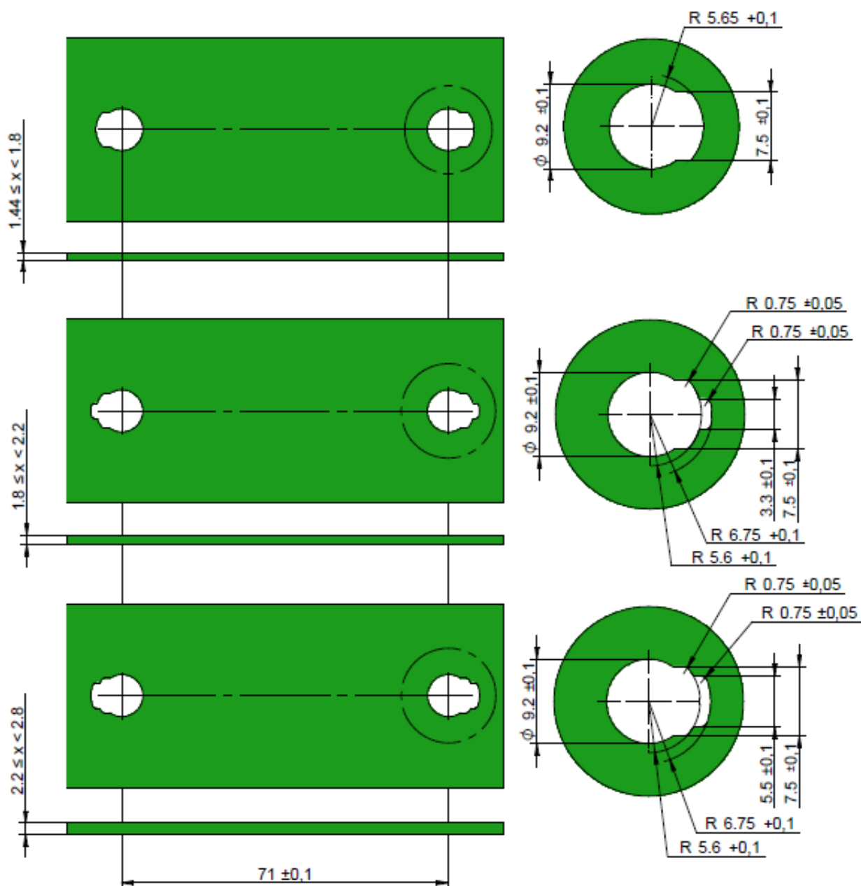
7. Figure PCB-cutouts for two-clip modules which are soldered, at various board thicknesses
