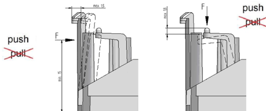
34. Figure: Permitted deformation of the clips and springs
