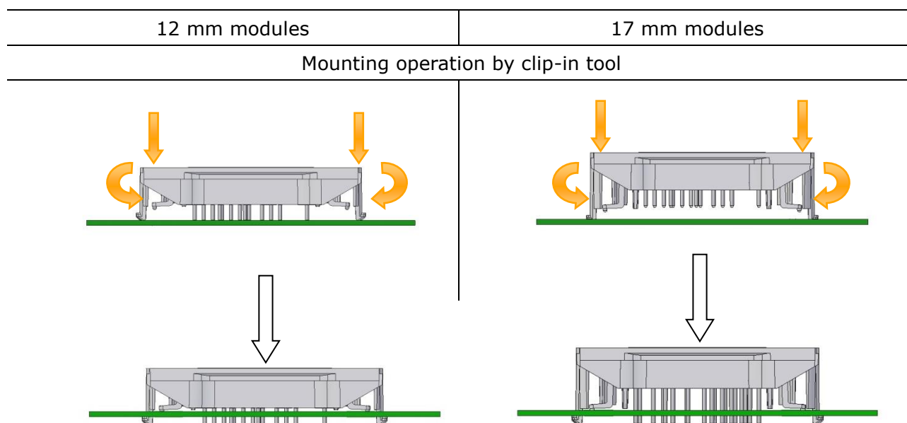
31. Figure: Mounting operation provided by the clip-in tool
