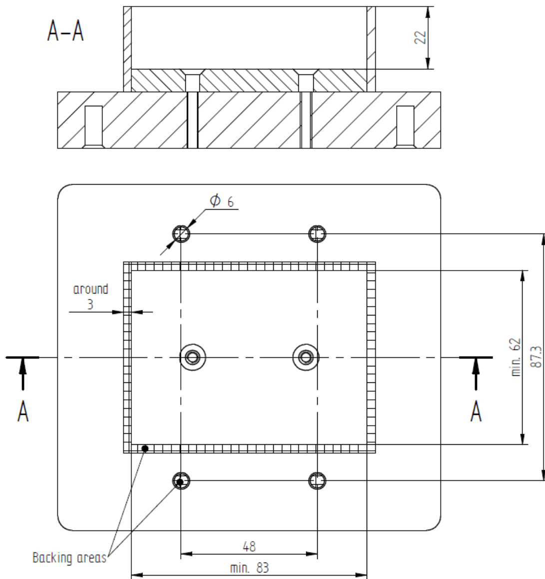
20. Figure Recommended dimensions of the lower tool
