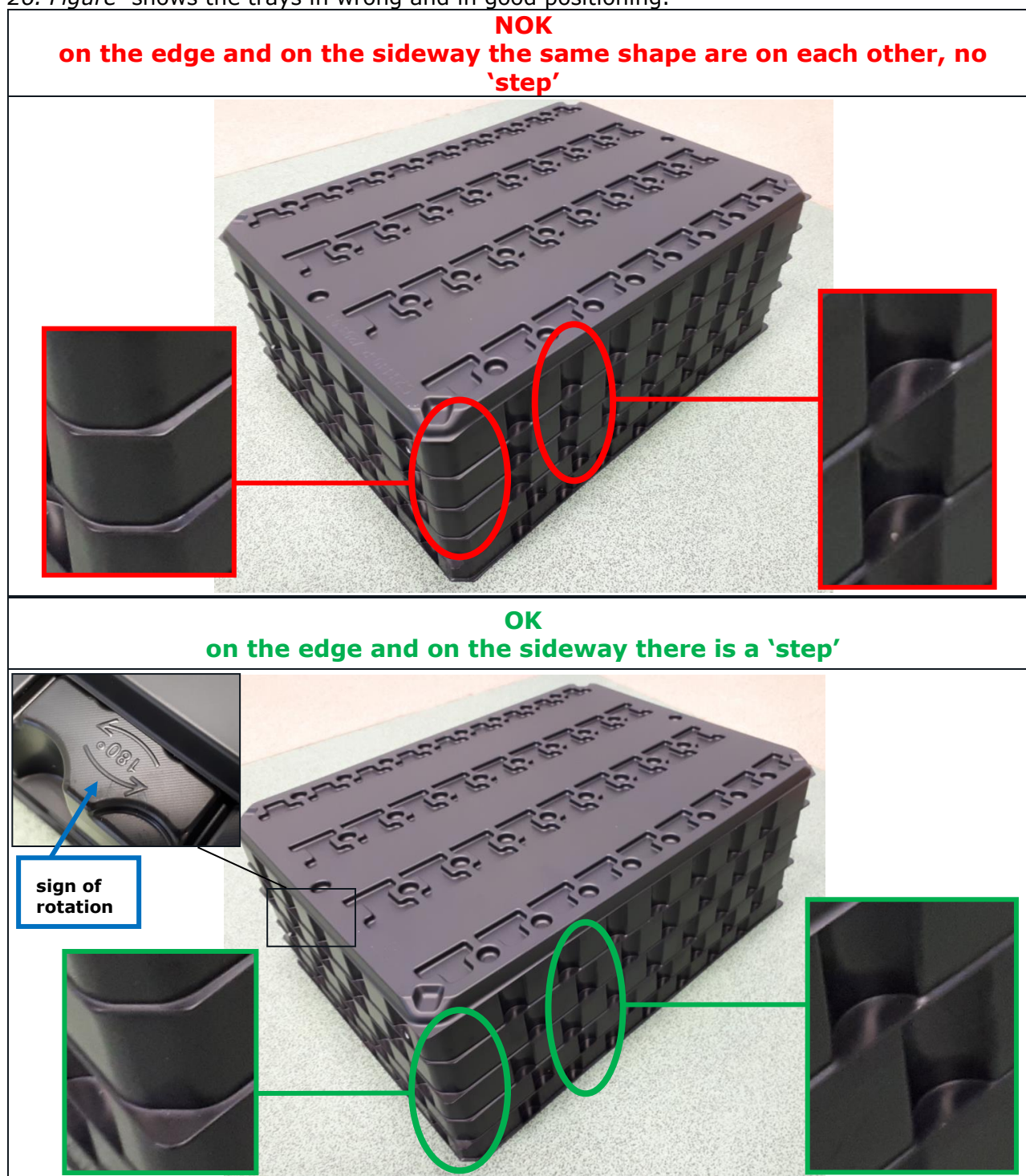
26. Figure Layer of trays
