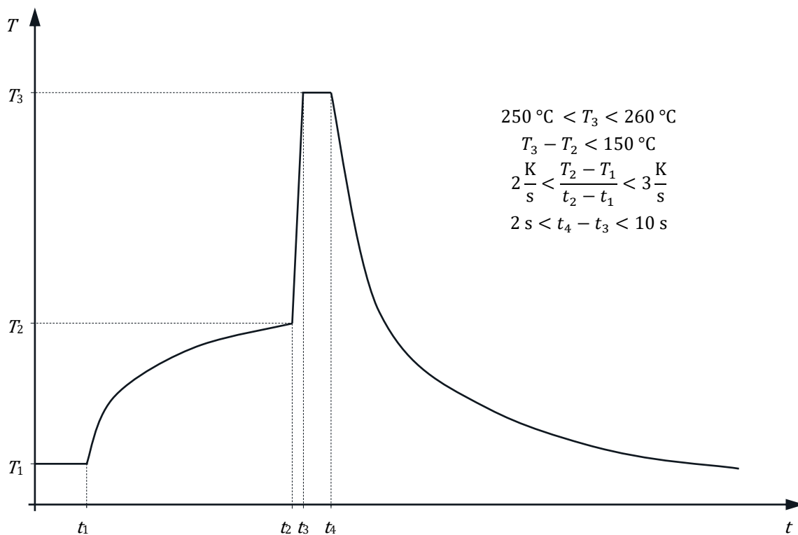
Figure 28: Typical profile for wave soldering
