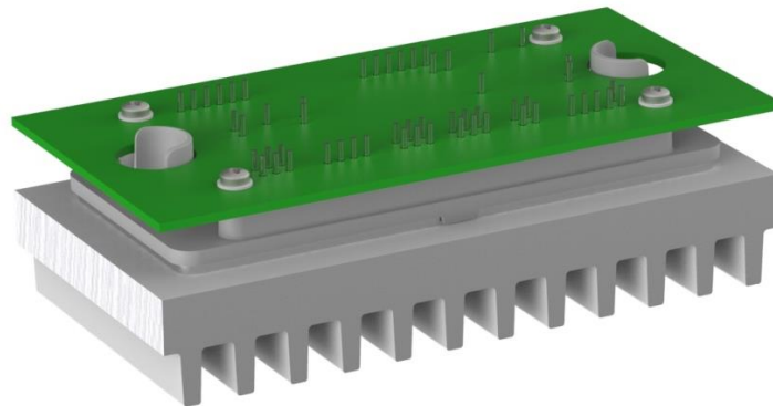
Figure 26: Assembly illustration
