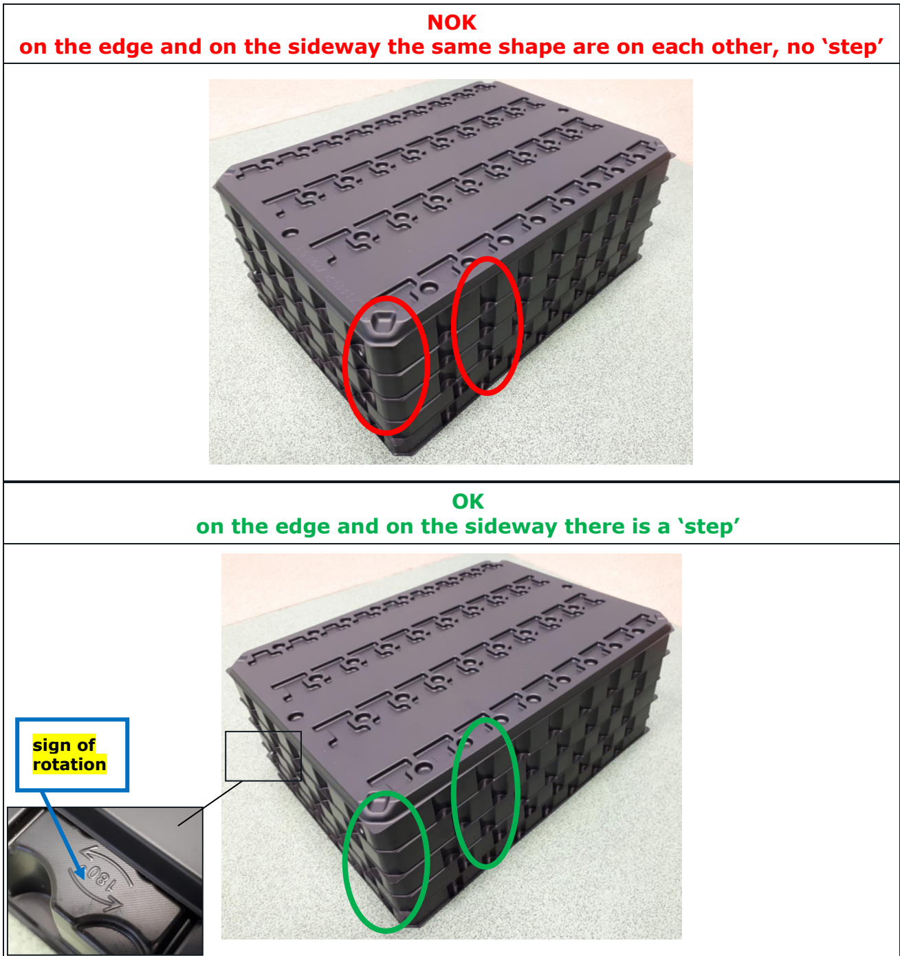
Figure 29: Layer of trays
