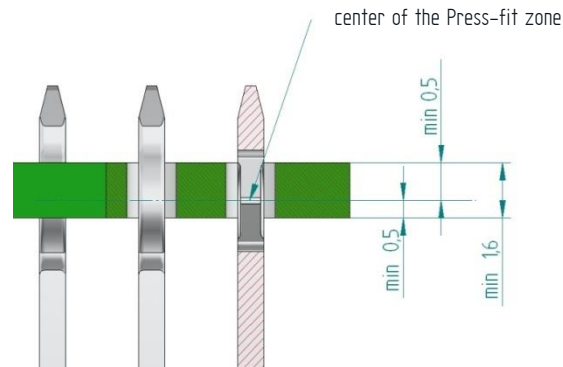
Figure 18: Press-in depth in PCB
