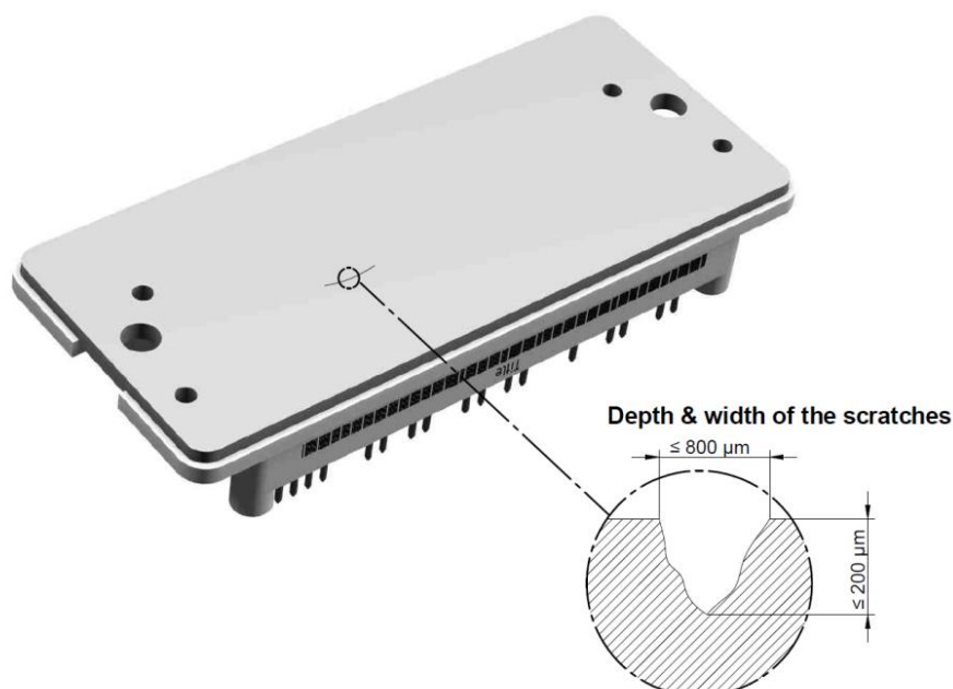
Figure 8: Scratch dimensions
