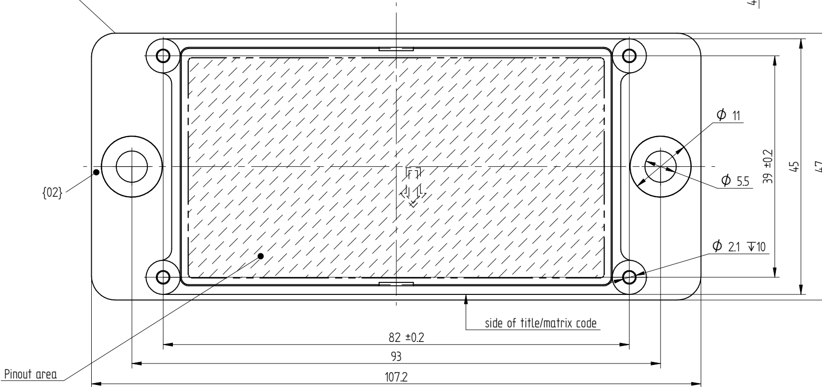
TOP VIEW WITHOUT PCB
