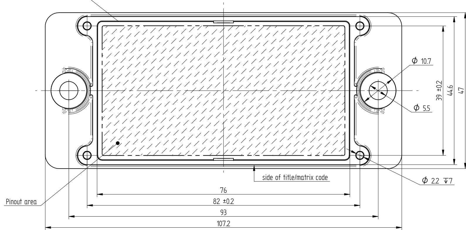
TOP VIEW WITHOUT PCB
