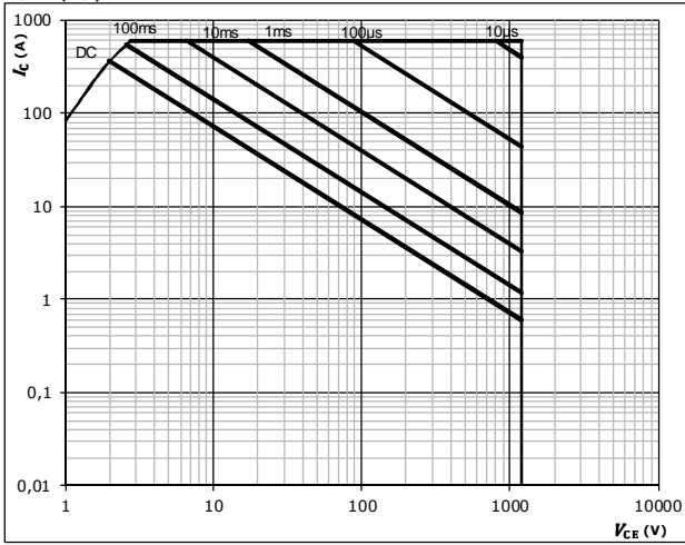
figure 5. IGBT
