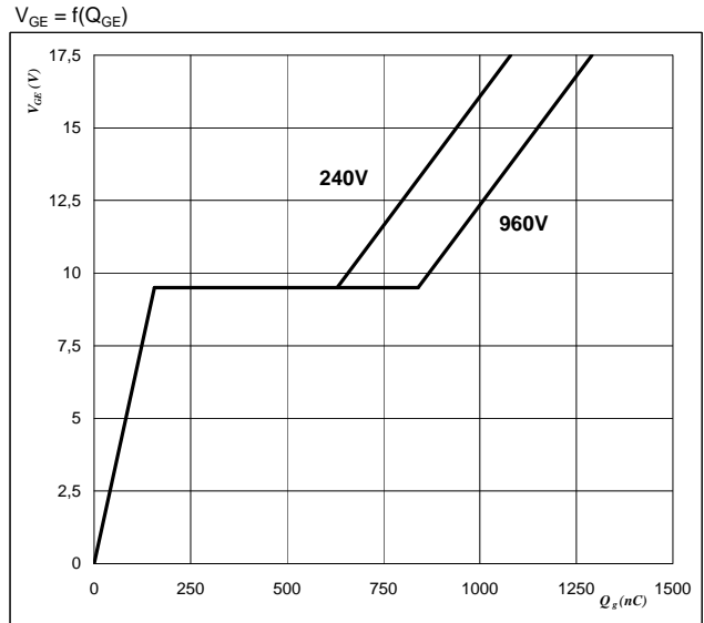
Figure 26 T1a,b,c-T6a,b,c IGBT
