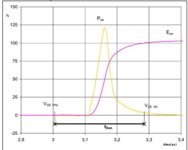
Figure 6 T1a,b,c-T6a,b,c IGBT Turn-on Switching Waveforms & definition of t_{Eon}
