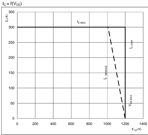
Figure 29 T1a,b,c-T6a,b,c IGBT
