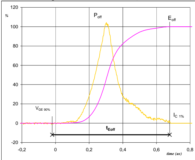
Figure 5 T1a,b,c-T6a,b,c IGBT Turn-off Switching Waveforms & definition of t_{Eoff}
