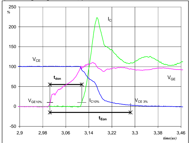
Figure 2 T1a,b,c-T6a,b,c IGBT
