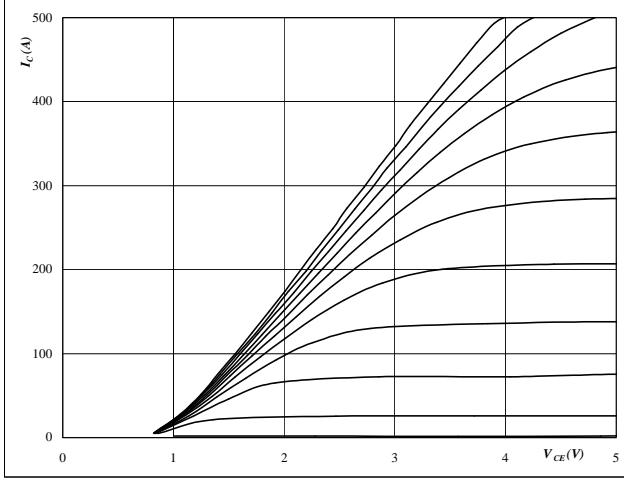
Figure 1 T1a,b,c-T6a,b,c IGBT
