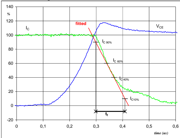
Figure 3 T1a,b,c-T6a,b,c IGBT
