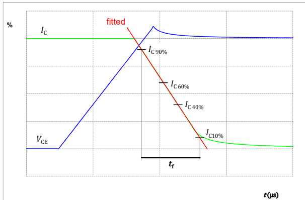
figure 52. IGBT Turn-off Switching Waveforms & definition of t_f
