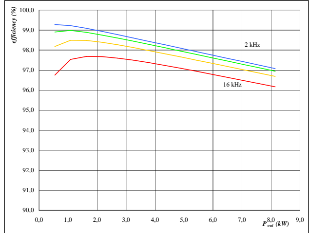
figure 10. Inverter Typical efficiency as a function of output power efficiency = f(P_{out})
