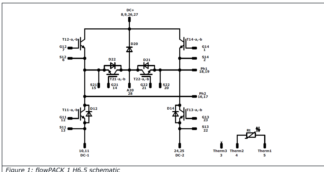
Figure 1: flowPACK 1 H6.5 schematic
