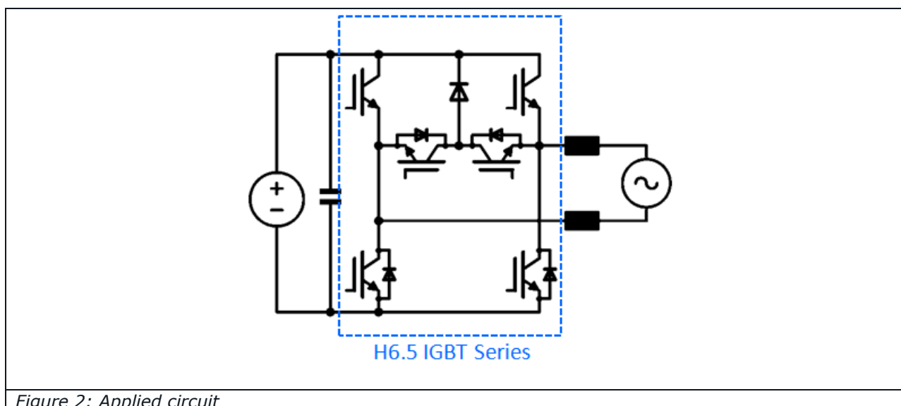
Figure 2: Applied circuit
