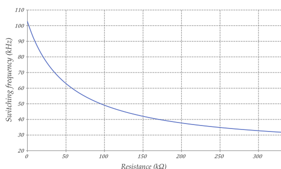
Figure 5: PFC switching frequency as a function of external resistance
