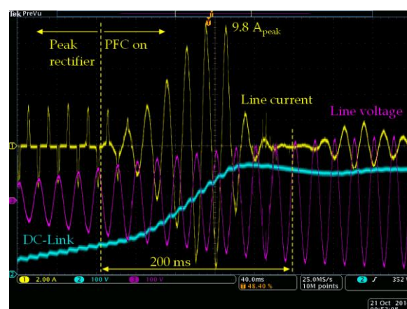
Figure 27: PFC startup with a slow input voltage increase (startup threshold = 75 V RMS )
