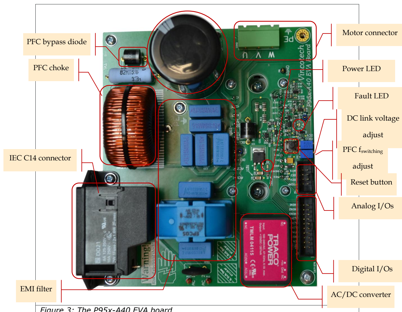
Figure 3: The P95x-A40 EVA board
