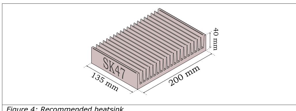
Figure 4: Recommended heatsink
