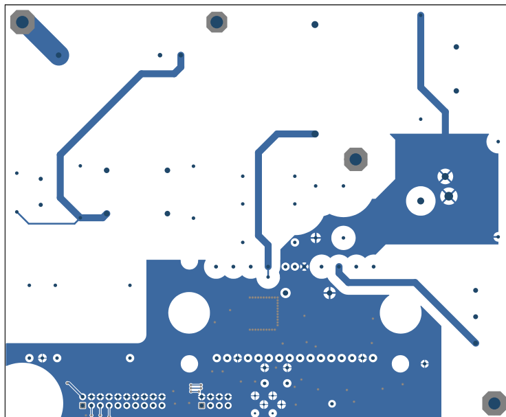
Figure 41: Bottom layer
