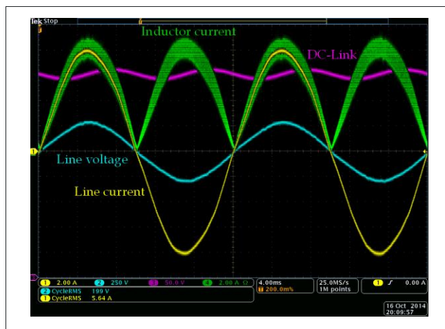
Figure 26: General PFC waveforms at full load ( V_{in} = 200 \text{ V}_{RMS} , P_{out} = 1000 \text{ W} )
