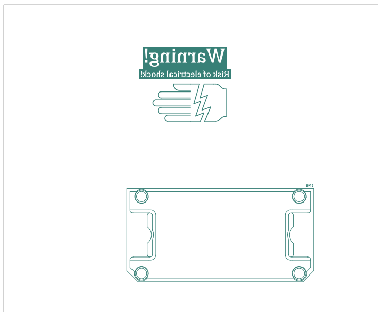
Figure 42: Bottom silkscreen
