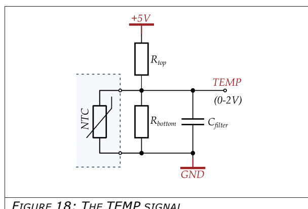
FIGURE 18: THE TEMP SIGNAL
