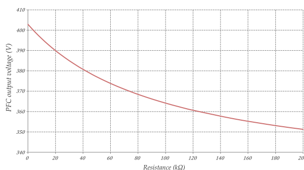
Figure 6: DC link voltage as a function of external resistance
