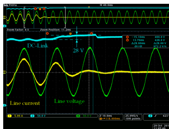
Figure 34: Load jump ( V_{in} = 100\text{ V} , P_{out} from 500 W to 0 W)
